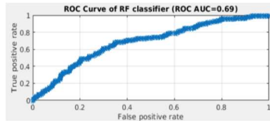
Figure 3. The ROC curve of the RF classifier. The ROC curve is generated by plotting the true positive rate (y-axis; TP/(TP+FN) ) against the false positive rate (x-axis; FP/(FP+TN) ). The true and false positive rates evaluate the accuracy of the model's classifications. It is the probability in which the model correctly or incorrectly classifies the individual respectively. The TOI has a ROC AUC of 0.69.
