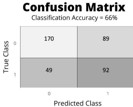
Figure 2. The confusion matrix. There are two axes: (1) the true class (y-axis; determined by blood samples), and (2) the predicted class (x-axis; determined by TOI). Non-diabetes is classified as '0', and diabetes is classified as '1'. The equal error rate (EER) threshold values for the model's false positive and false negative rate is set to {159 100 55 86 } 0.351. TOI has a classification accuracy of 66%.
